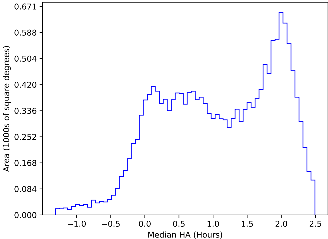
too_elab_heavy_r128_d2_ugrizy_v3.4_10yrs WFD u band: Median HA
