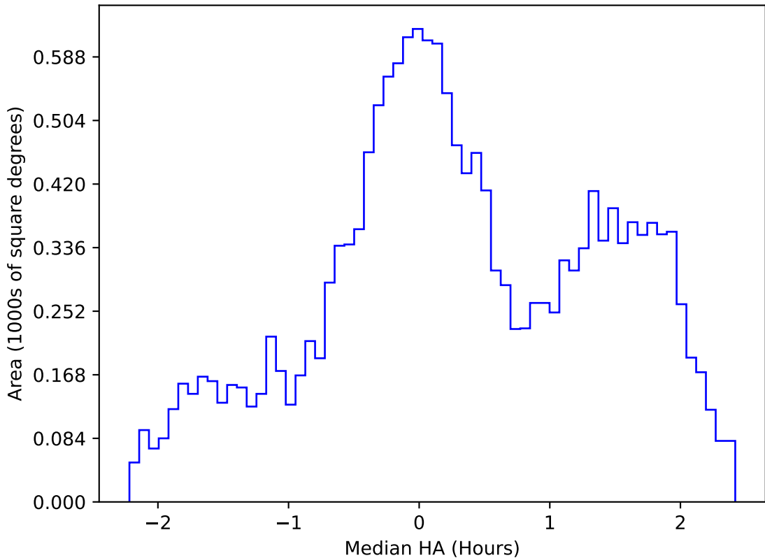
too_elab_heavy_r128_d2_ugrizy_v3.4_10yrs WFD g band: Median HA
