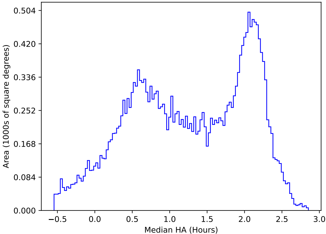
too_elab_heavy_r128_d2_ugrizy_v3.4_10yrs All sky y band: Median HA
