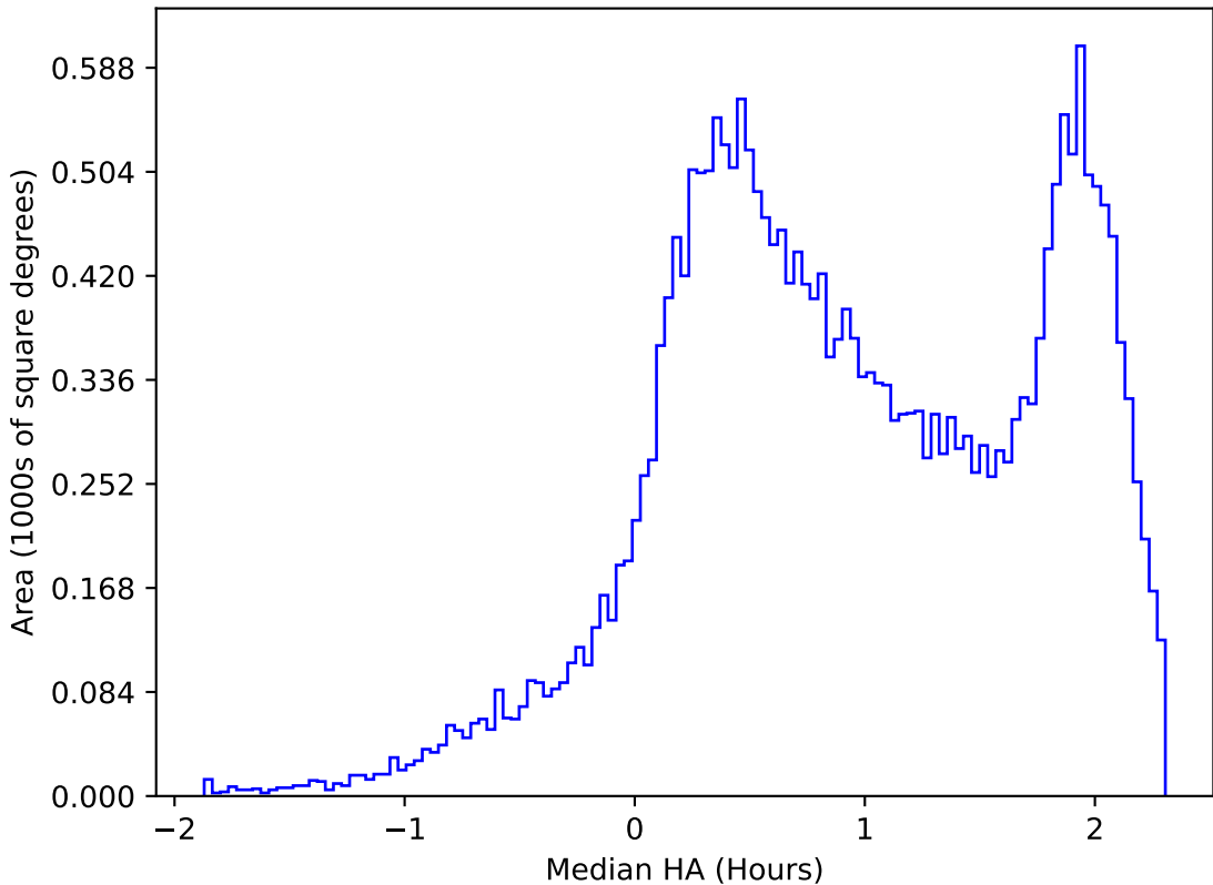
too_elab_heavy_r128_d2_ugrizy_v3.4_10yrs All sky i band: Median HA
