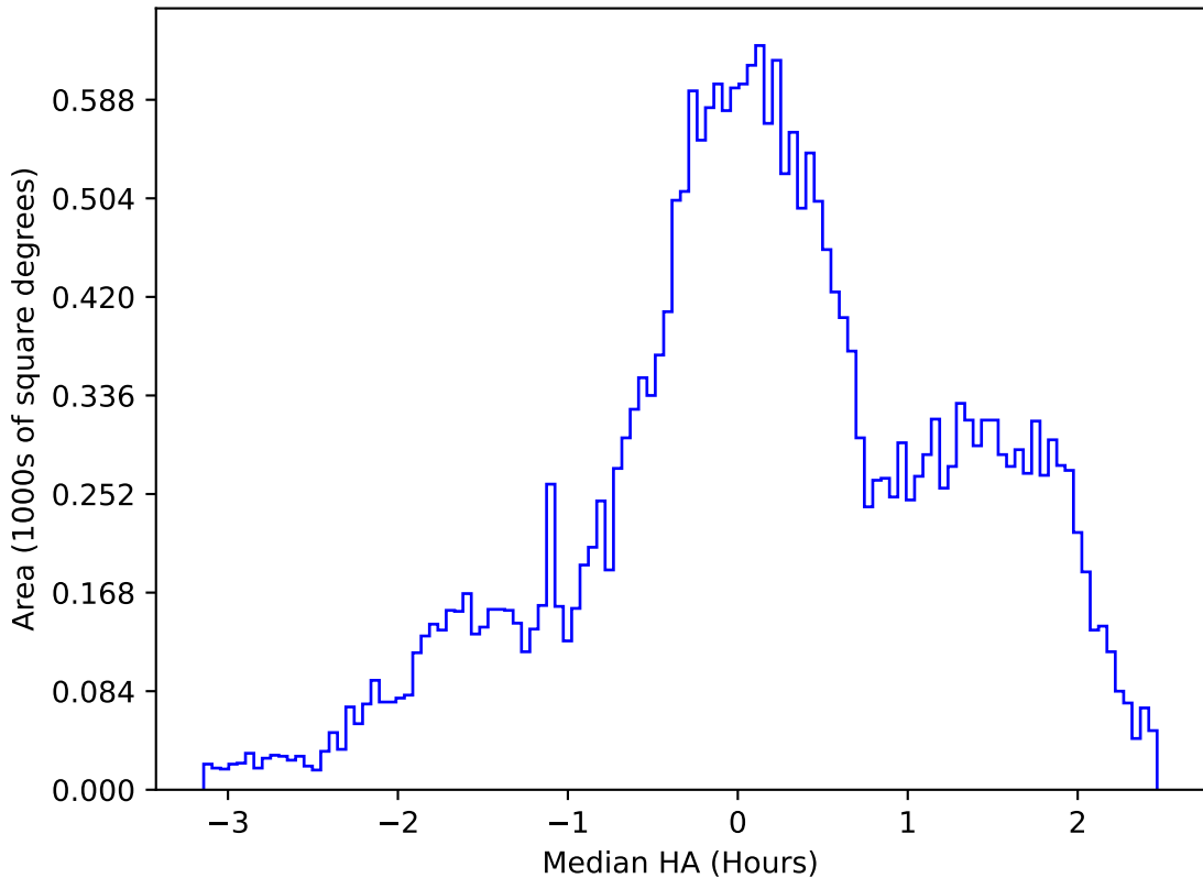
too_elab_heavy_r128_d2_ugrizy_v3.4_10yrs All sky g band: Median HA
