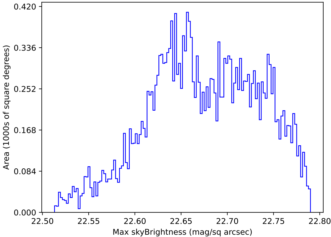
too_elab_heavy_r128_d2_ugrizy_v3.4_10yrs Yr 1 u band: Max skyBrightness
