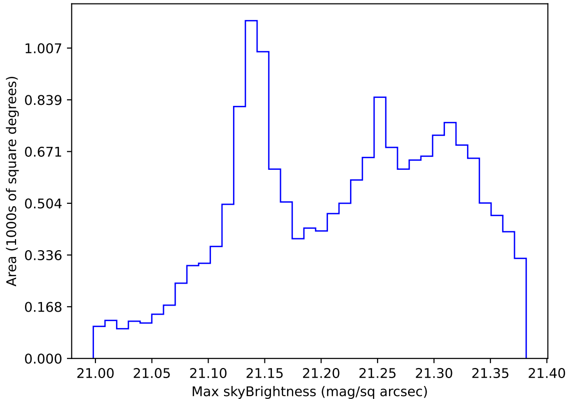
too_elab_heavy_r128_d2_ugrizy_v3.4_10yrs WFD r band: Max skyBrightness
