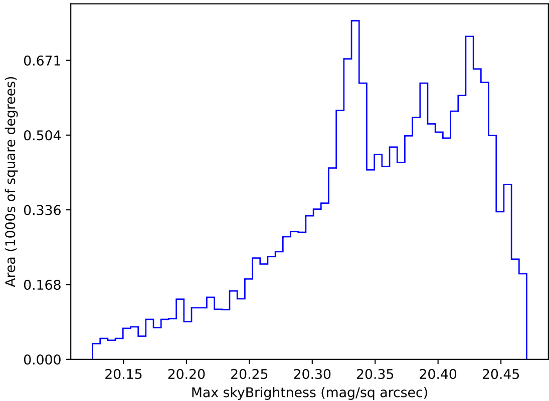
too_elab_heavy_r128_d2_ugrizy_v3.4_10yrs WFD i band: Max skyBrightness
