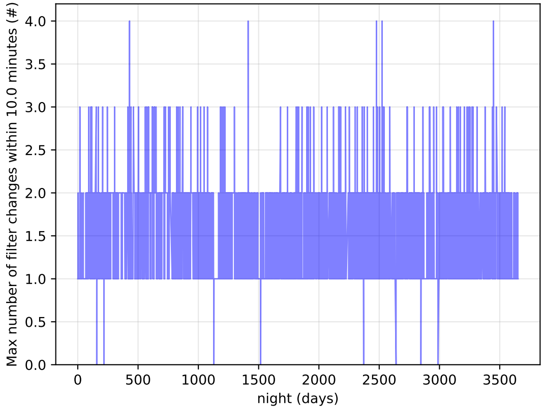
too_elab_heavy_r128_d2_ugrizy_v3.4_10yrs Per Night: Max number of filter changes within 10.0 minutes
