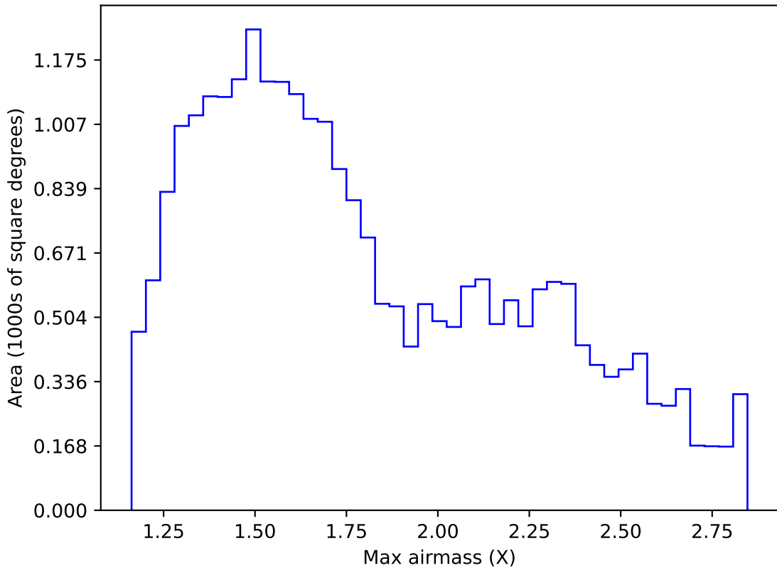
too_elab_heavy_r128_d2_ugrizy_v3.4_10yrs Yr 1 z band: Max airmass
