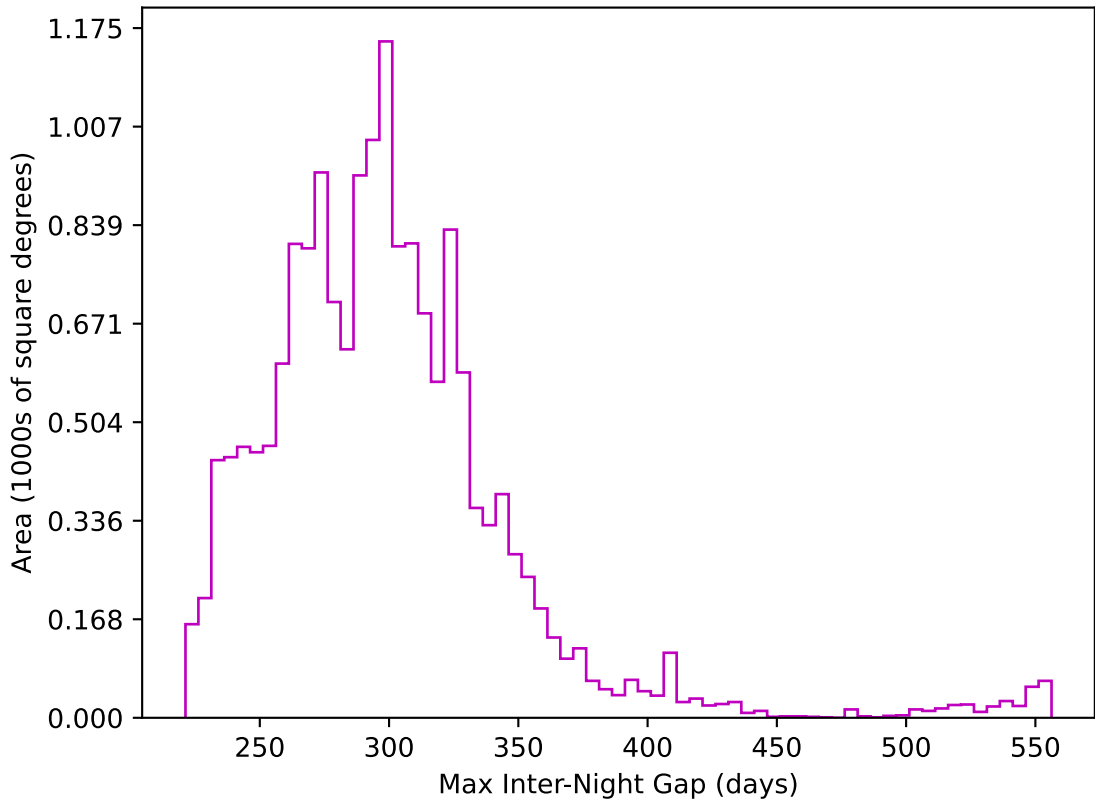
too_elab_heavy_r128_d2_ugrizy_v3.4_10yrs WFD z band: Max Inter-Night Gap
