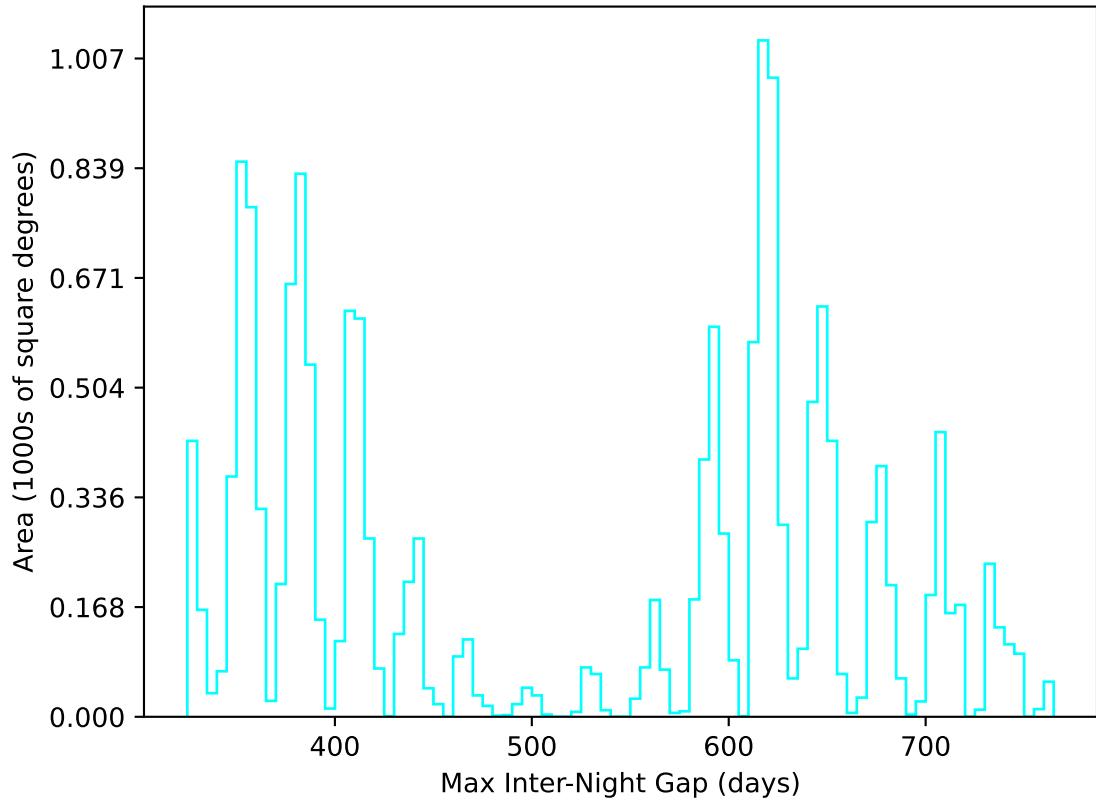
too_elab_heavy_r128_d2_ugrizy_v3.4_10yrs WFD u band: Max Inter-Night Gap
