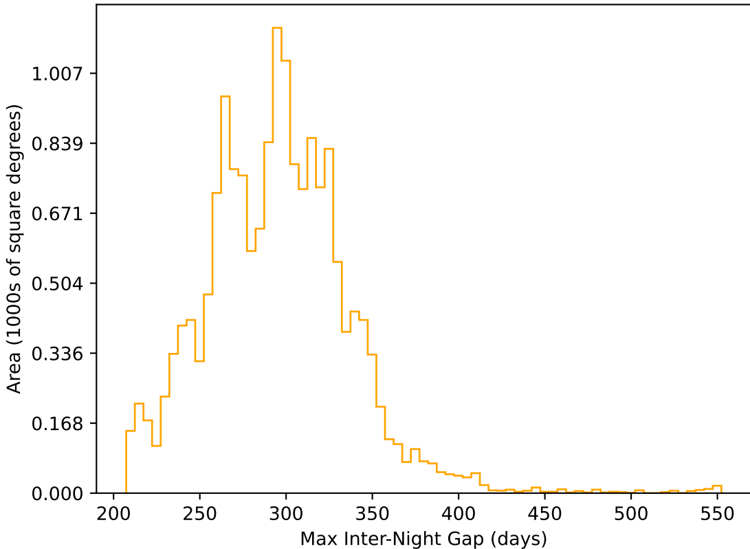
too_elab_heavy_r128_d2_ugrizy_v3.4_10yrs WFD r band: Max Inter-Night Gap
