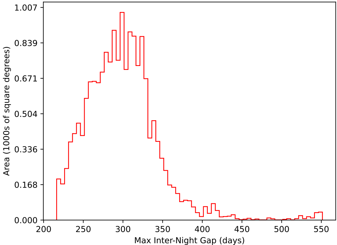
too_elab_heavy_r128_d2_ugrizy_v3.4_10yrs WFD i band: Max Inter-Night Gap
