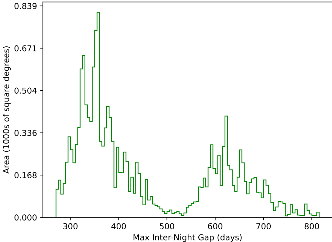
too_elab_heavy_r128_d2_ugrizy_v3.4_10yrs WFD g band: Max Inter-Night Gap
