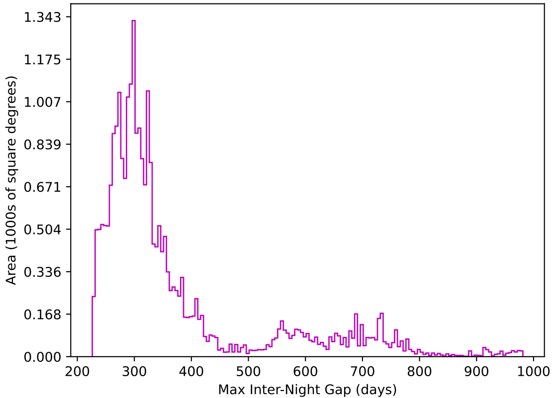
too_elab_heavy_r128_d2_ugrizy_v3.4_10yrs All sky z band: Max Inter-Night Gap
