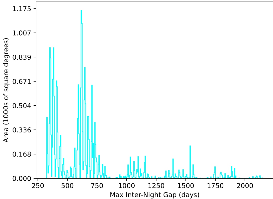
too_elab_heavy_r128_d2_ugrizy_v3.4_10yrs All sky u band: Max Inter-Night Gap
