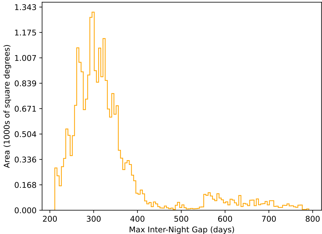
too_elab_heavy_r128_d2_ugrizy_v3.4_10yrs All sky r band: Max Inter-Night Gap
