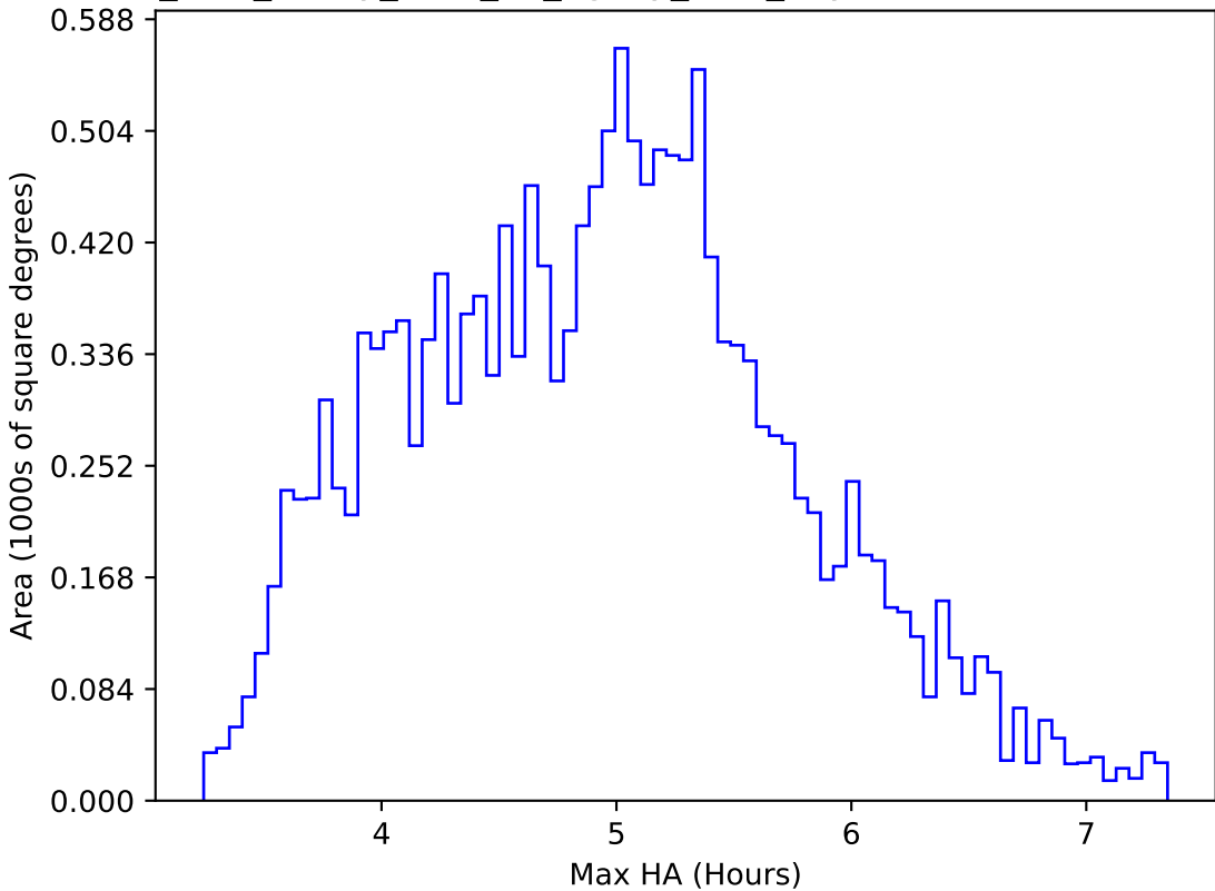
too_elab_heavy_r128_d2_ugrizy_v3.4_10yrs WFD z band: Max HA
