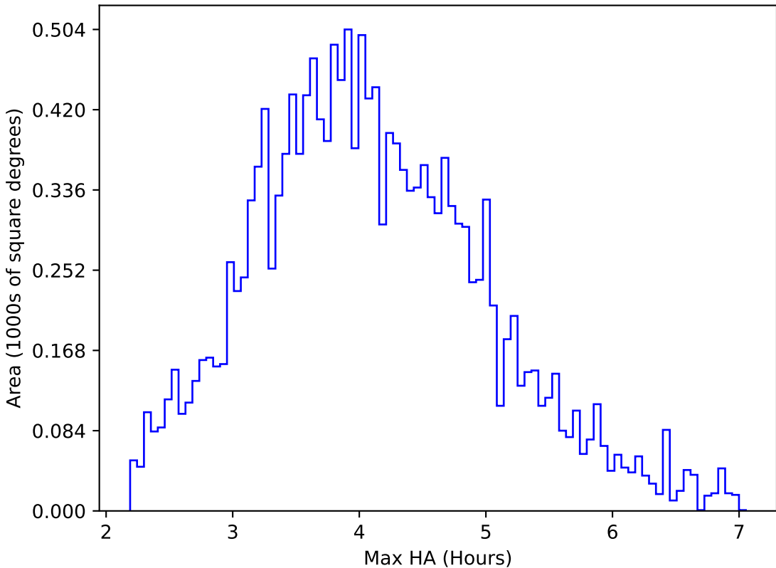
too_elab_heavy_r128_d2_ugrizy_v3.4_10yrs WFD u band: Max HA
