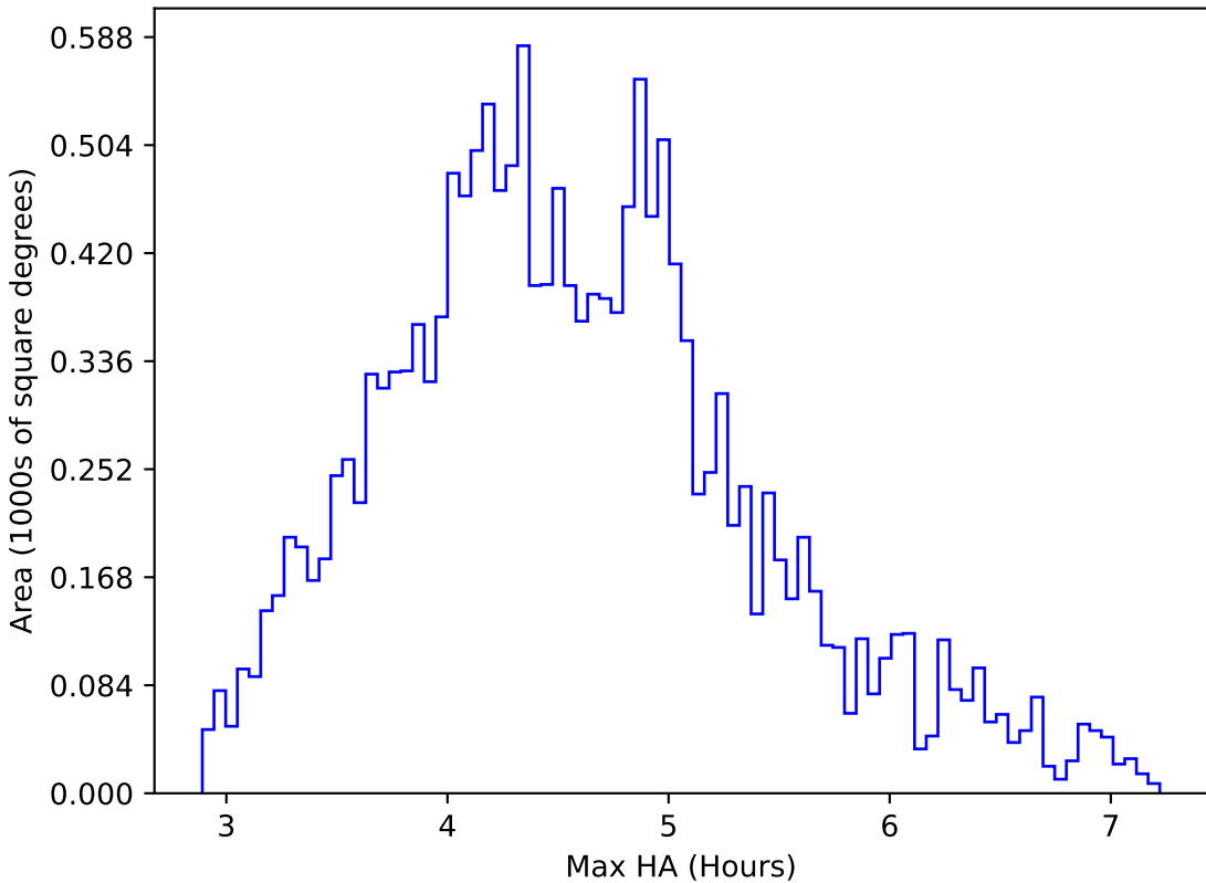
too_elab_heavy_r128_d2_ugrizy_v3.4_10yrs WFD r band: Max HA
