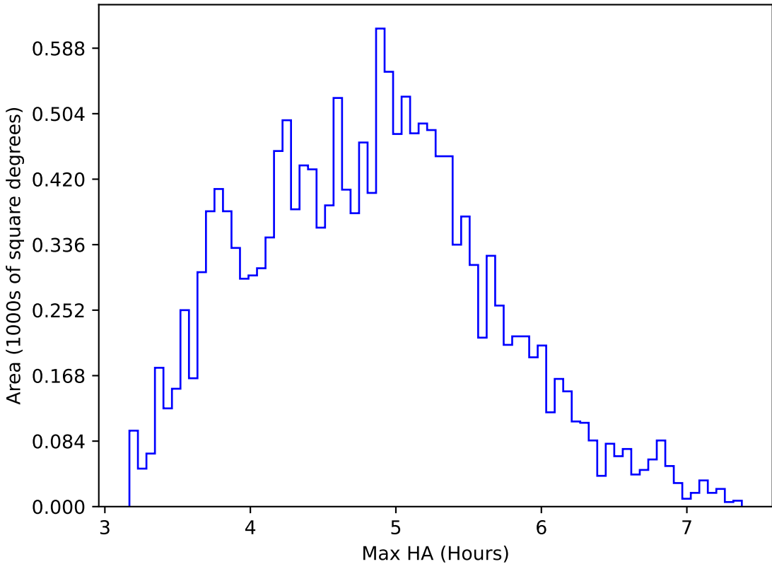
too_elab_heavy_r128_d2_ugrizy_v3.4_10yrs WFD i band: Max HA
