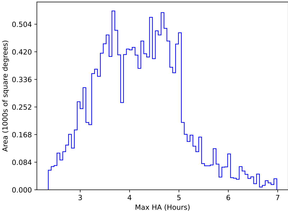
too_elab_heavy_r128_d2_ugrizy_v3.4_10yrs WFD g band: Max HA
