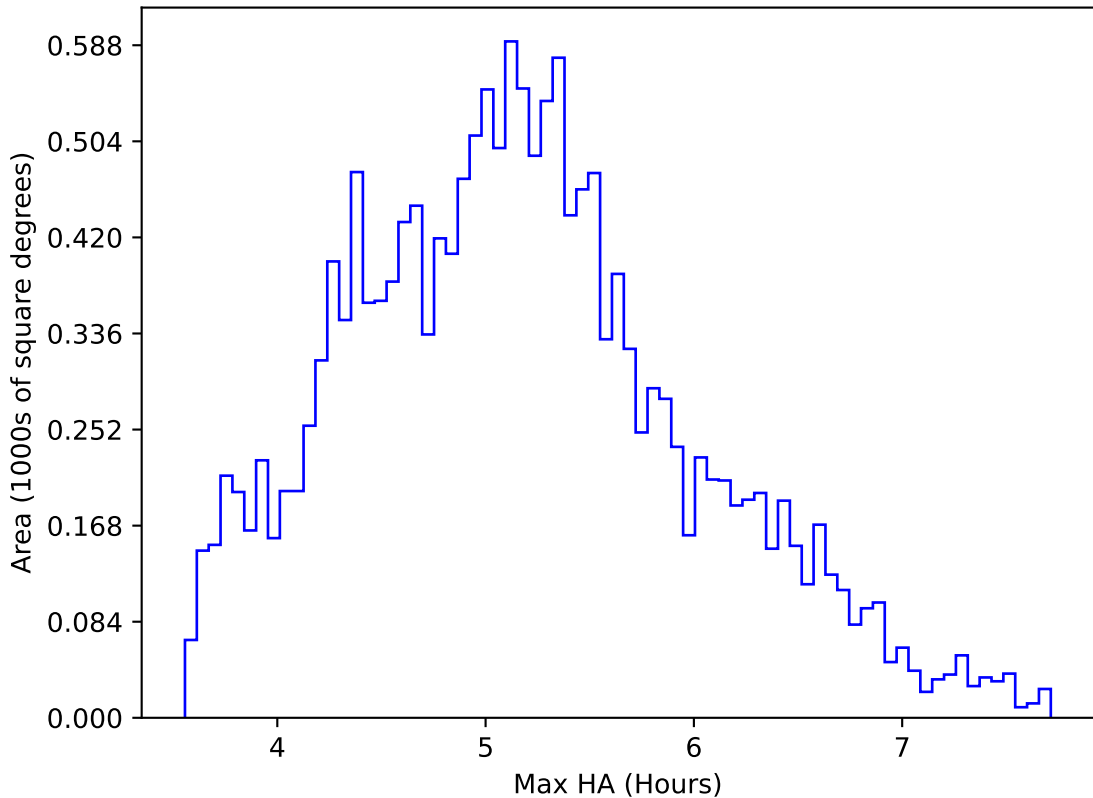
too_elab_heavy_r128_d2_ugrizy_v3.4_10yrs WFD all bands: Max HA
