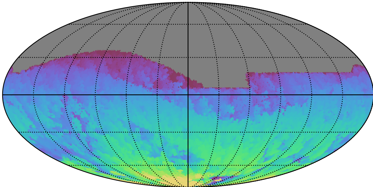
too_elab_heavy_r128_d2_ugrizy_v3.4_10yrs All sky z band: Max HA
