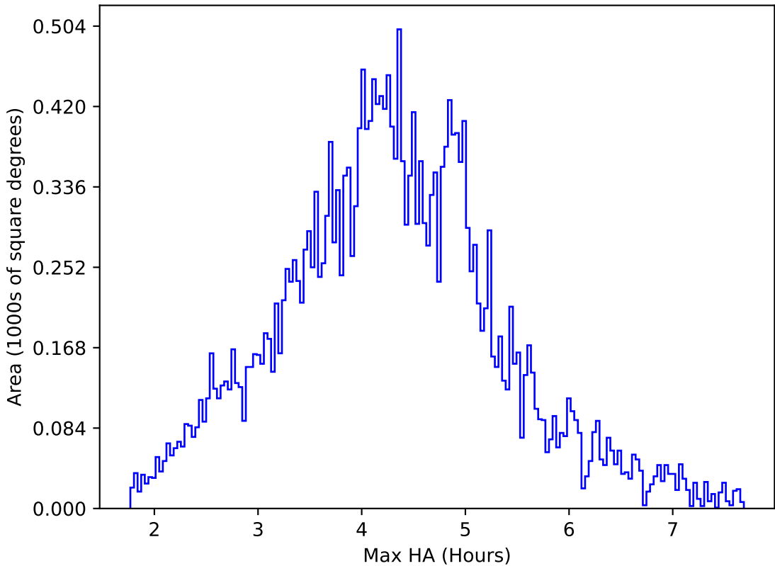
too_elab_heavy_r128_d2_ugrizy_v3.4_10yrs All sky r band: Max HA
