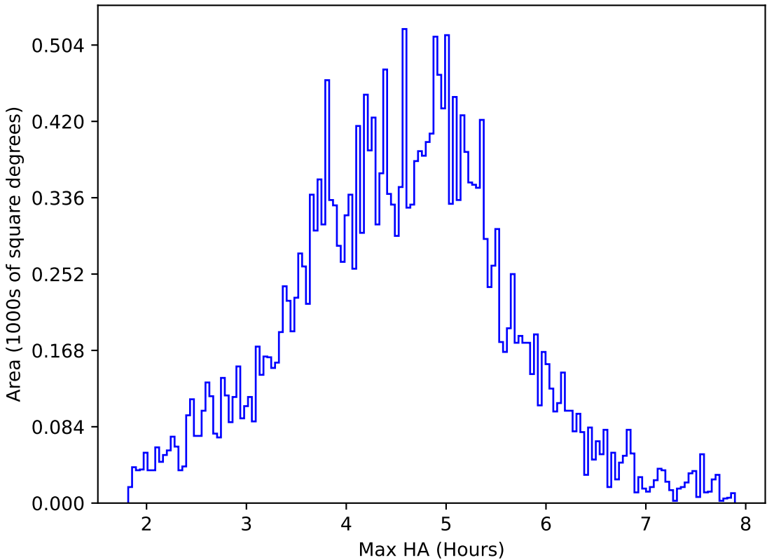
too_elab_heavy_r128_d2_ugrizy_v3.4_10yrs All sky i band: Max HA
