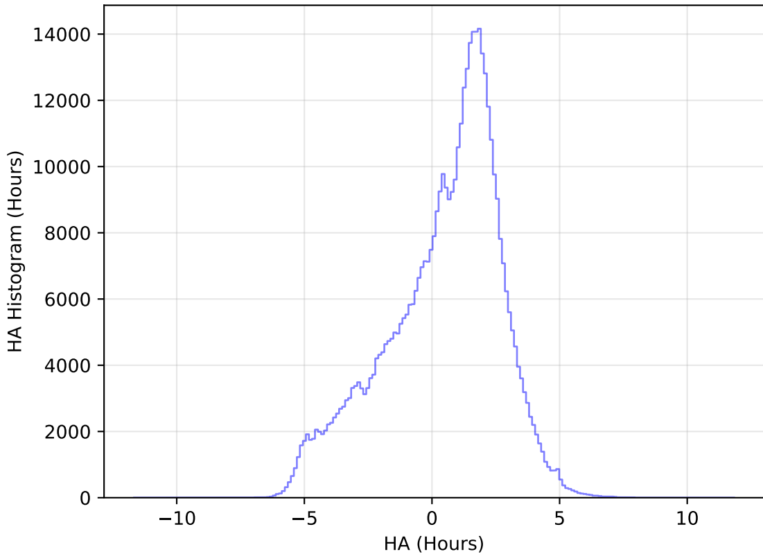
too_elab_heavy_r128_d2_ugrizy_v3.4_10yrs WFD r band: HA Histogram
