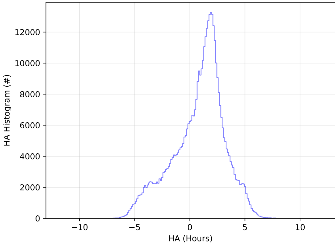
too_elab_heavy_r128_d2_ugrizy_v3.4_10yrs All sky z band: HA Histogram
