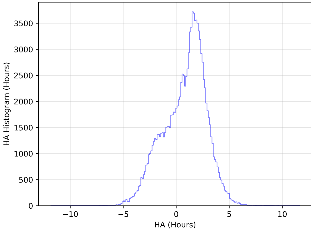
too_elab_heavy_r128_d2_ugrizy_v3.4_10yrs All sky u band: HA Histogram
