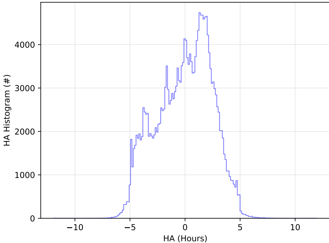
too_elab_heavy_r128_d2_ugrizy_v3.4_10yrs All sky g band: HA Histogram
