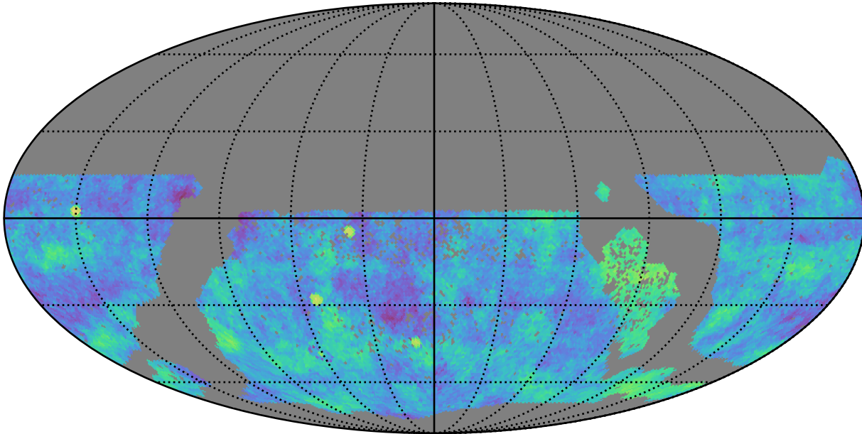
too_elab_heavy_r128_d2_ugrizy_v3.4_10yrs gri WFD: Fraction of visits in pairs (20-90 min)
