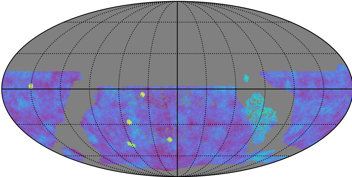
too_elab_heavy_r128_d2_ugrizy_v3.4_10yrs gri WFD: Fraction of visits in pairs (10-60 min)
