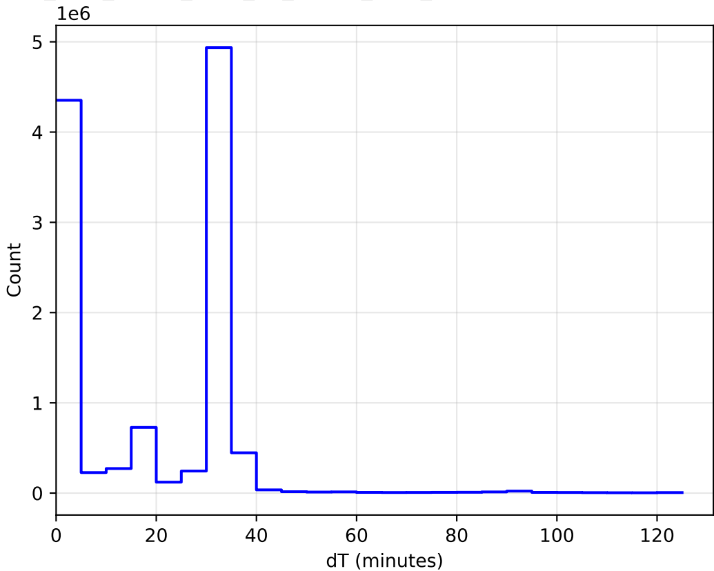
too_elab_heavy_r128_d2_ugrizy_v3.4_10yrs WFD: DeltaT Histogram
