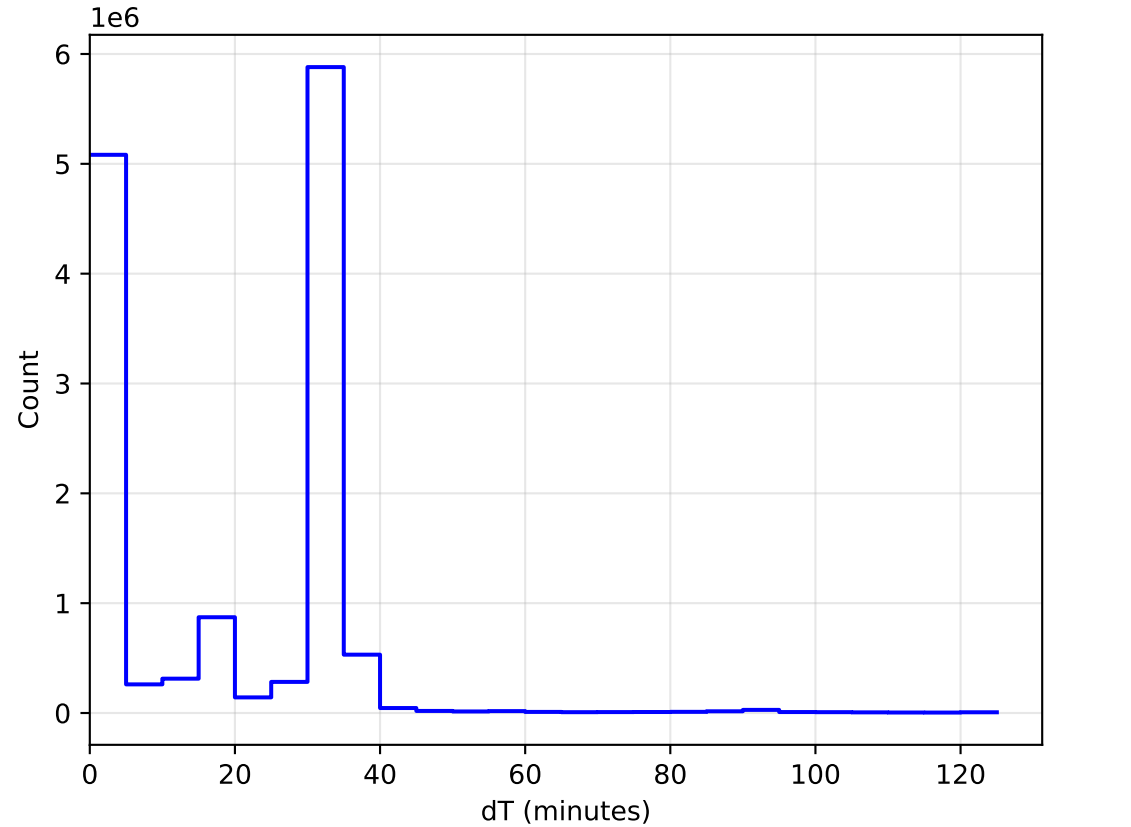
too_elab_heavy_r128_d2_ugrizy_v3.4_10yrs All sky: DeltaT Histogram
