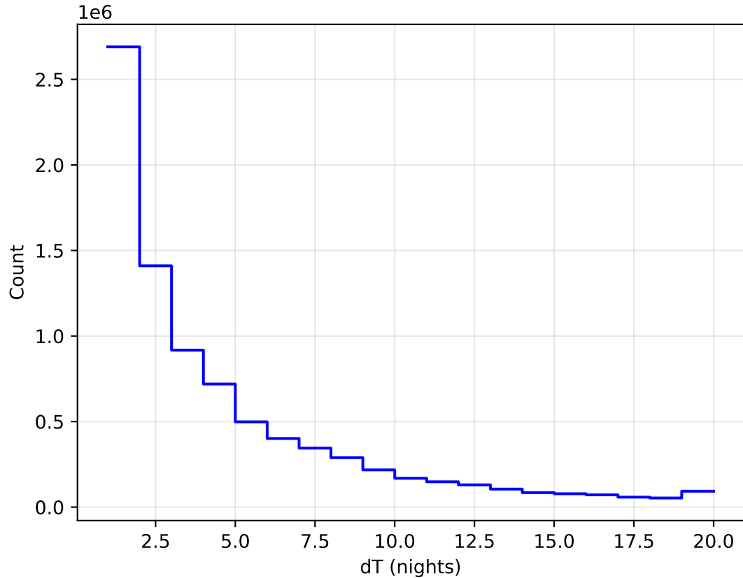
too_elab_heavy_r128_d2_ugrizy_v3.4_10yrs All sky all bands: DeltaNight Histogram
