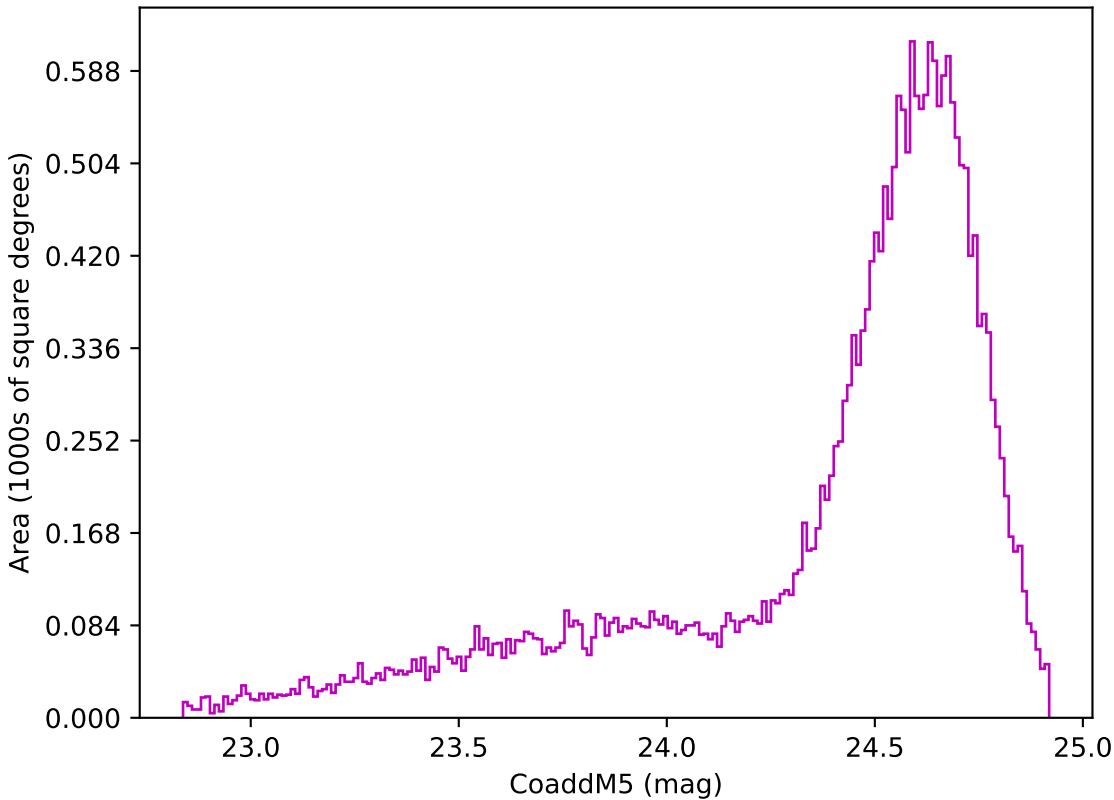
too_elab_heavy_r128_d2_ugrizy_v3.4_10yrs Yr 1 z band: CoaddM5
