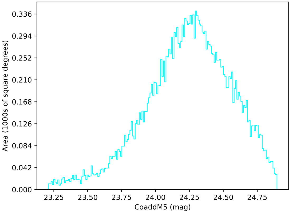
too_elab_heavy_r128_d2_ugrizy_v3.4_10yrs Yr 1 u band: CoaddM5
