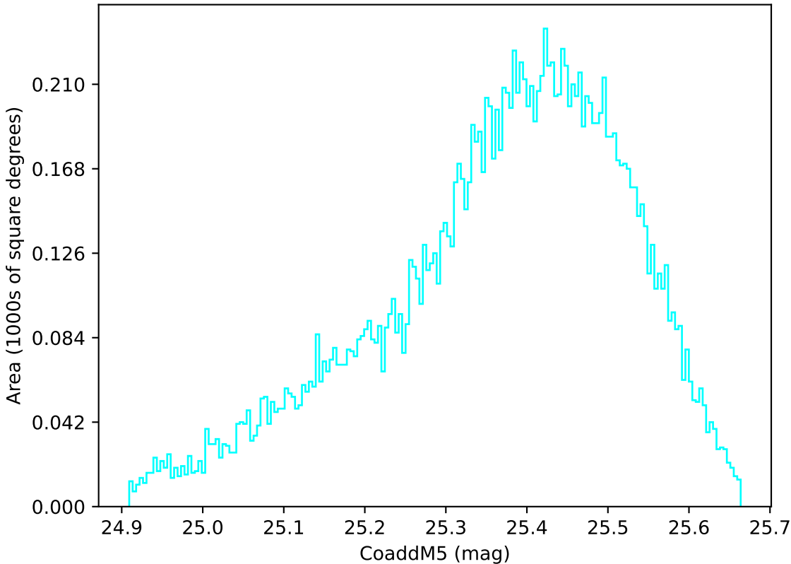
too_elab_heavy_r128_d2_ugrizy_v3.4_10yrs WFD u band: CoaddM5
