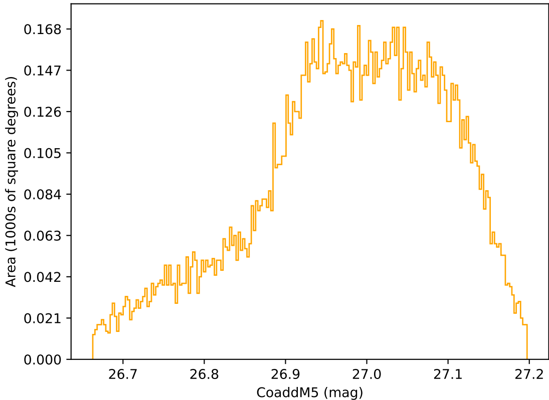
too_elab_heavy_r128_d2_ugrizy_v3.4_10yrs WFD r band: CoaddM5
