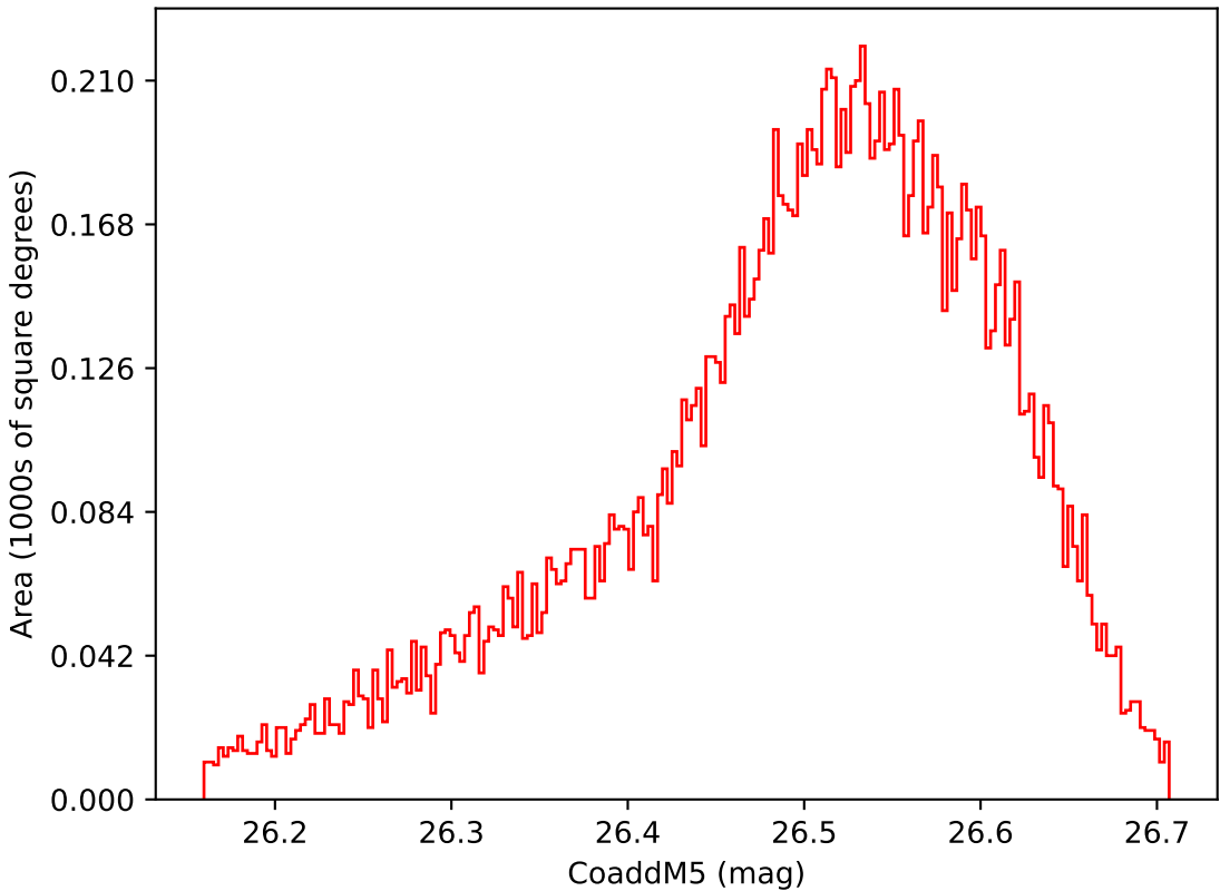
too_elab_heavy_r128_d2_ugrizy_v3.4_10yrs WFD i band: CoaddM5
