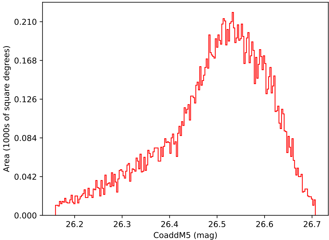
too_elab_heavy_r128_d2_ugrizy_v3.4_10yrs WFD i band: CoaddM5
