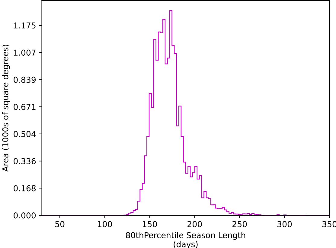
too_elab_heavy_r128_d2_ugrizy_v3.4_10yrs WFD z band: 80thPercentile Season Length
