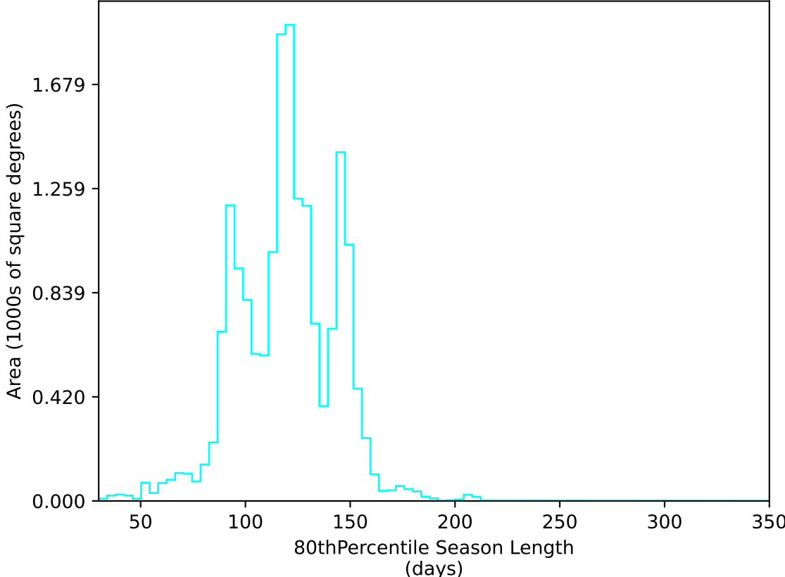
too_elab_heavy_r128_d2_ugrizy_v3.4_10yrs WFD u band: 80thPercentile Season Length
