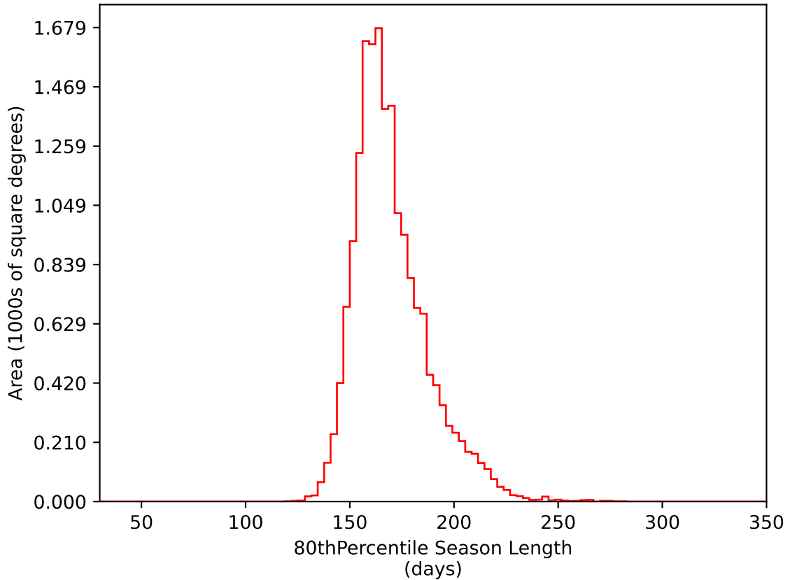
too_elab_heavy_r128_d2_ugrizy_v3.4_10yrs WFD i band: 80thPercentile Season Length
