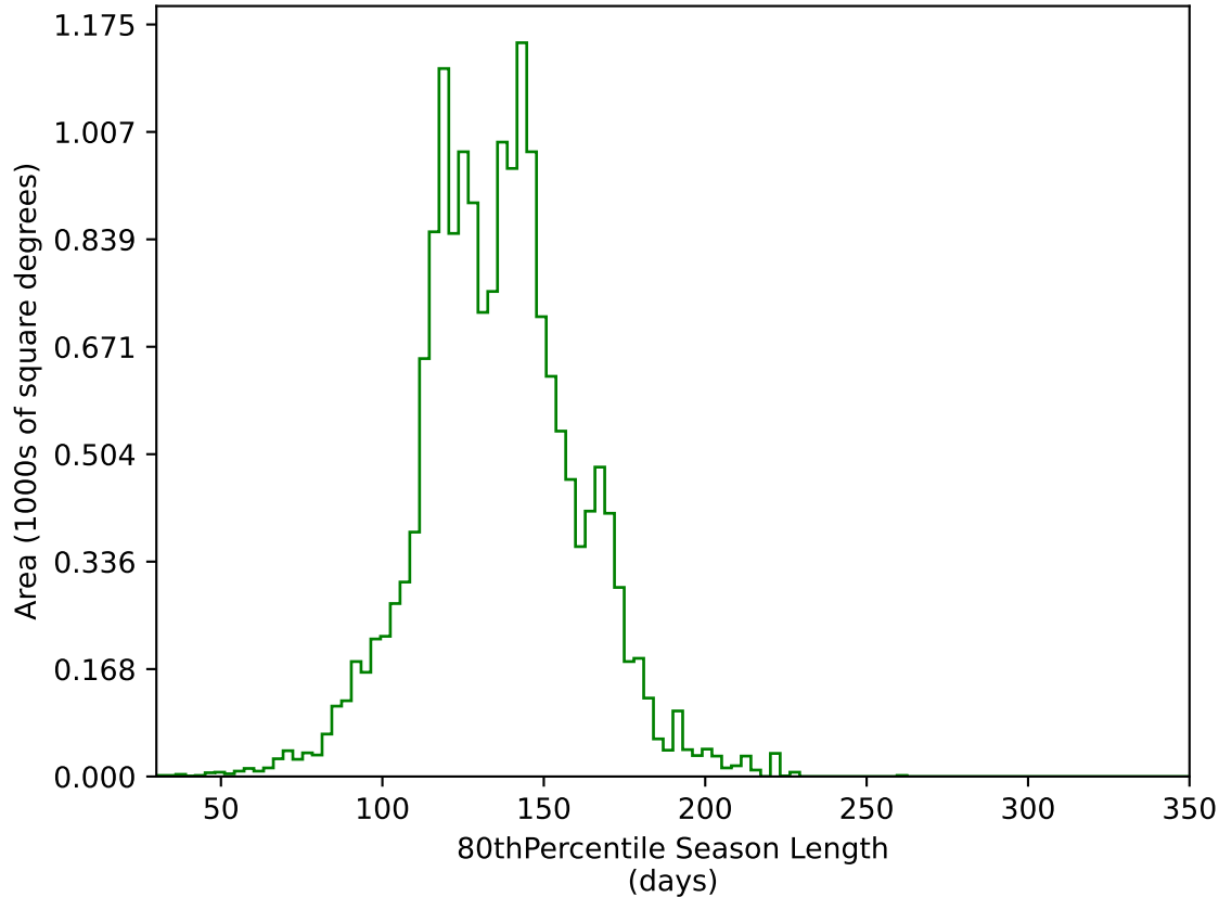
too_elab_heavy_r128_d2_ugrizy_v3.4_10yrs WFD g band: 80thPercentile Season Length
