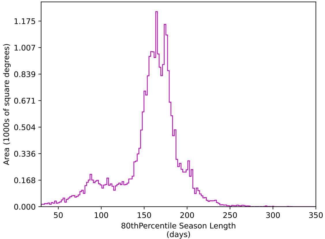
too_elab_heavy_r128_d2_ugrizy_v3.4_10yrs All sky z band: 80thPercentile Season Length
