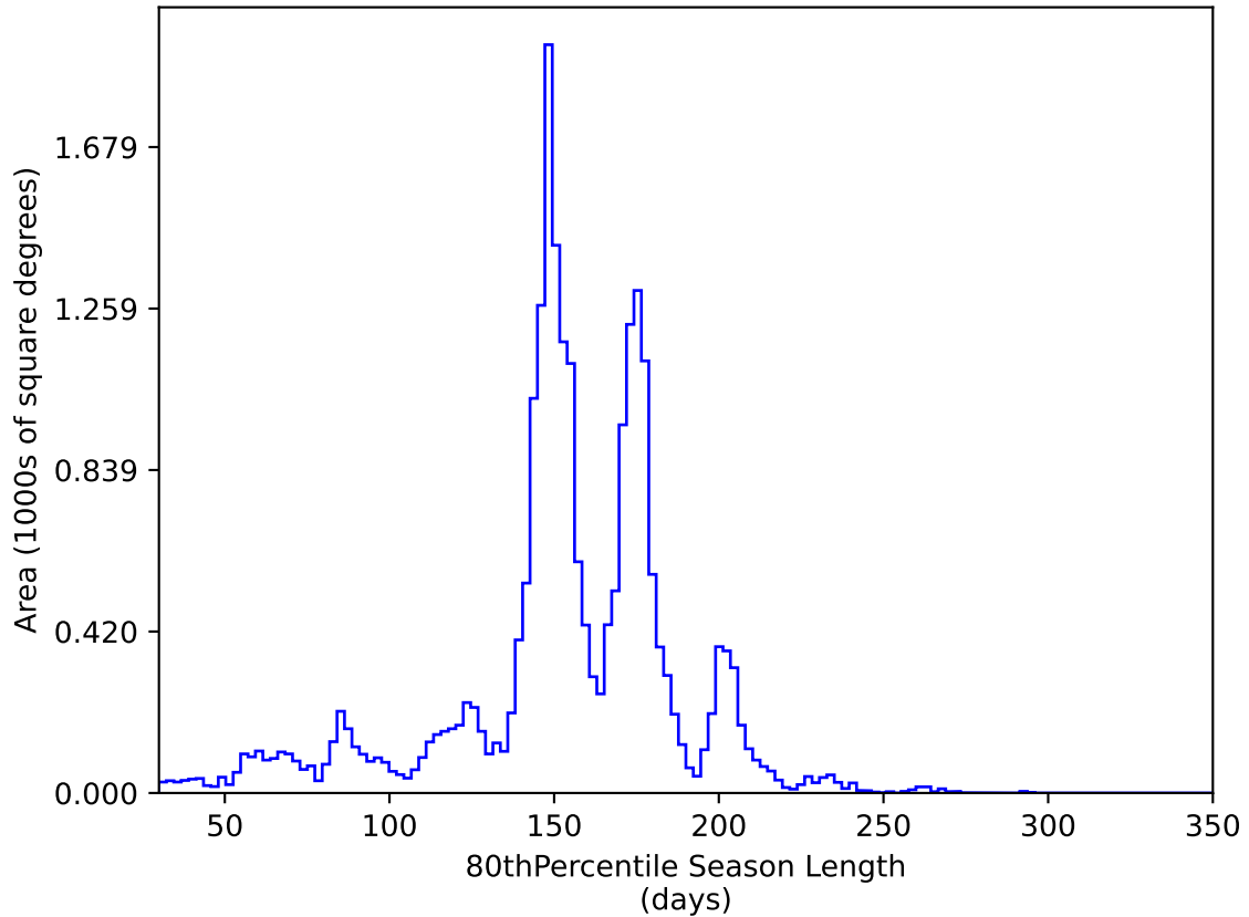
too_elab_heavy_r128_d2_ugrizy_v3.4_10yrs All sky y band: 80thPercentile Season Length
