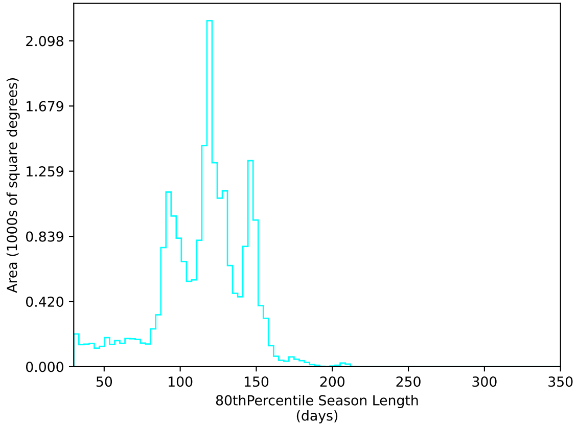
too_elab_heavy_r128_d2_ugrizy_v3.4_10yrs All sky u band: 80thPercentile Season Length
