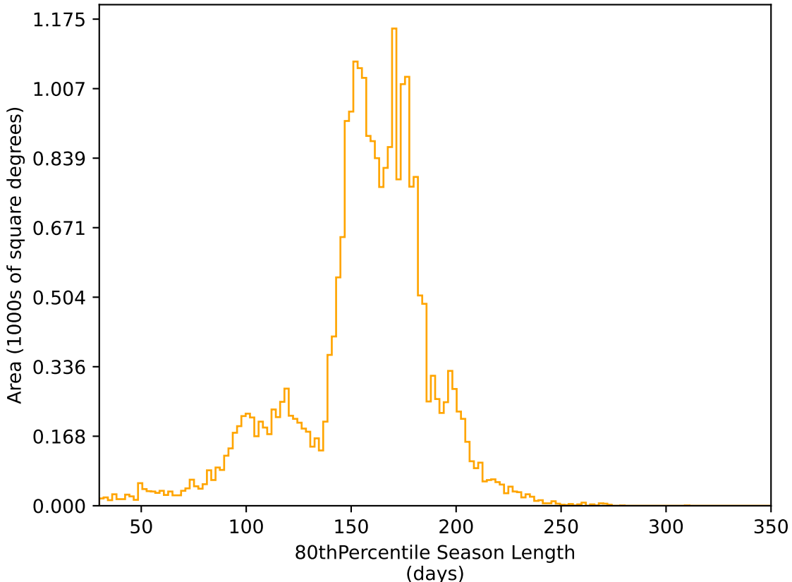
too_elab_heavy_r128_d2_ugrizy_v3.4_10yrs All sky r band: 80thPercentile Season Length
