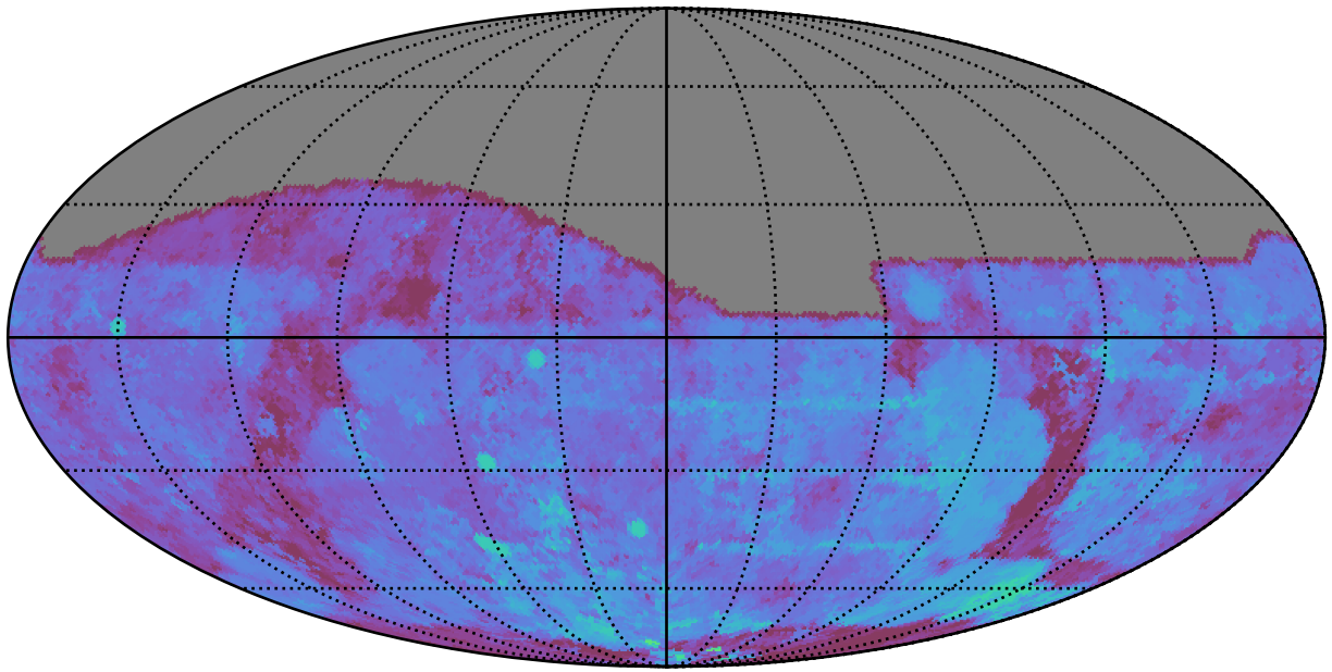
too_elab_heavy_r128_d2_ugrizy_v3.4_10yrs All sky g band: 80thPercentile Season Length
